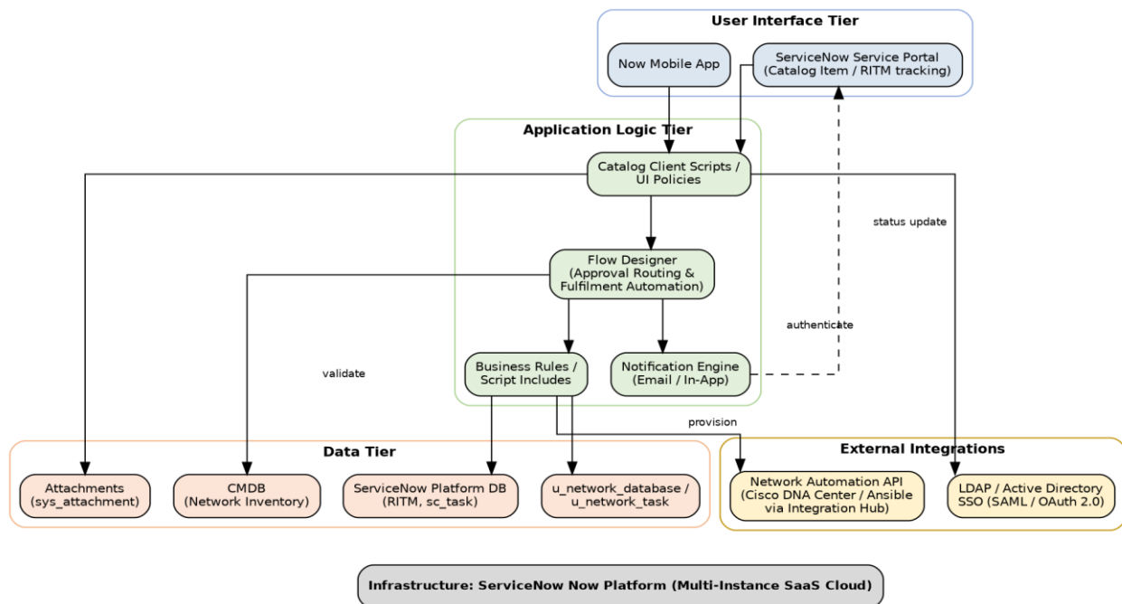
Figure 1: Technical Architecture – Automated Network Request Management (ServiceNow)
